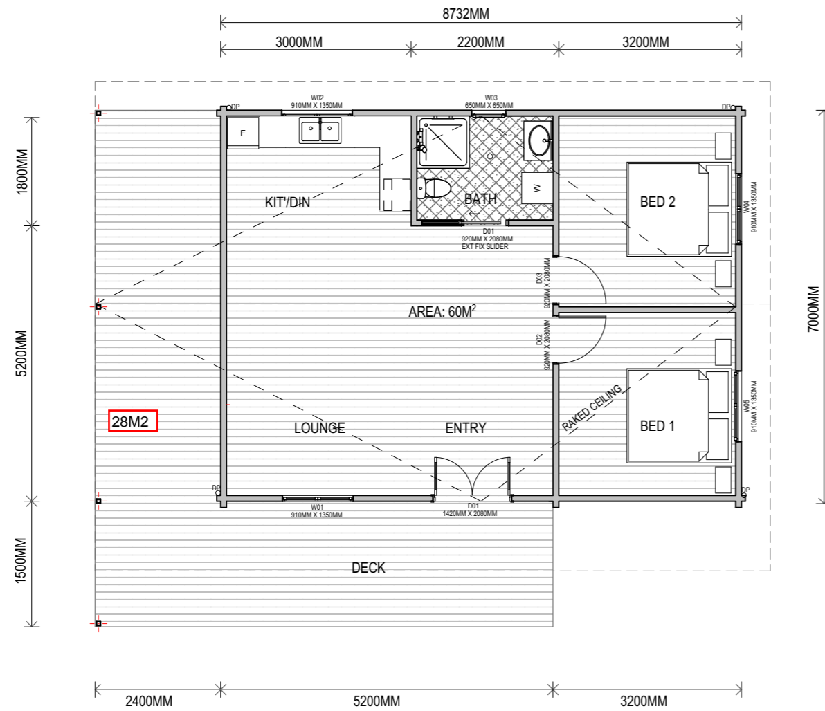
GROUND FLOOR 1:100
